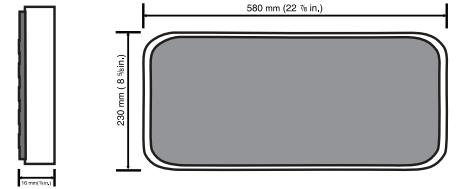
WALL MOUNTED FRAME
