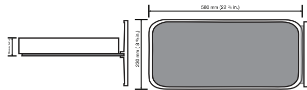
FLAG MOUNTED FRAME
