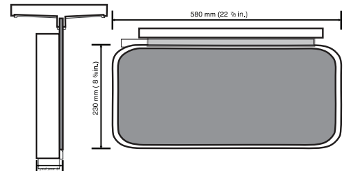
CEILING MOUNTED FRAME
